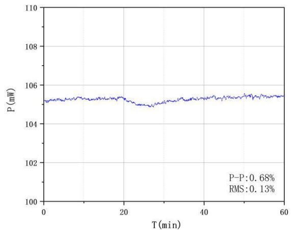
Power Stability @100mW
