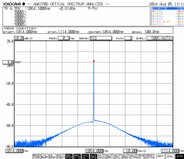
Optical Spectrum@ 100mW (After 20dB attenuation)
